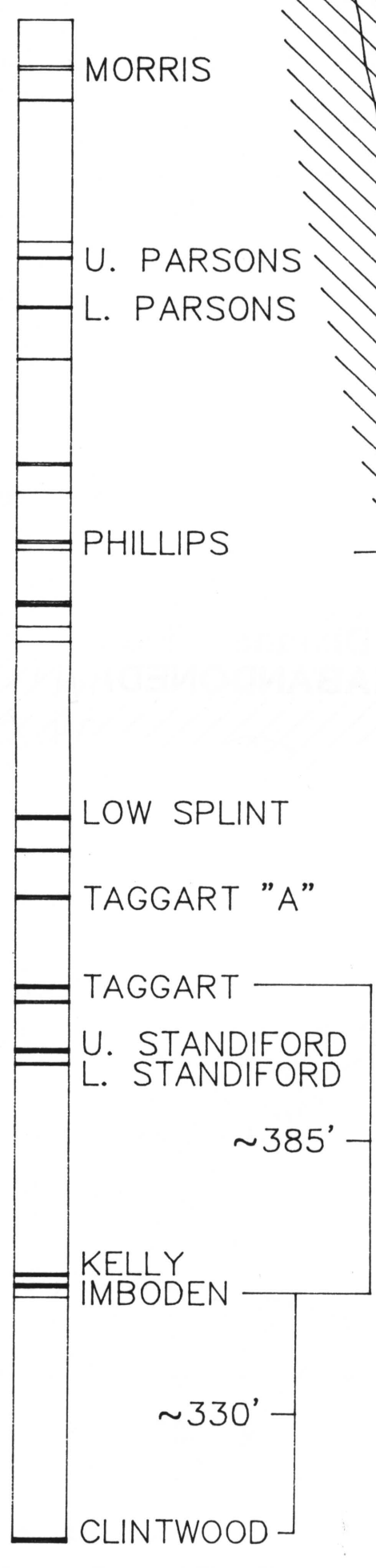
TYPICAL STRATIGRAPHIC COLUMN NOT TO SCALE
