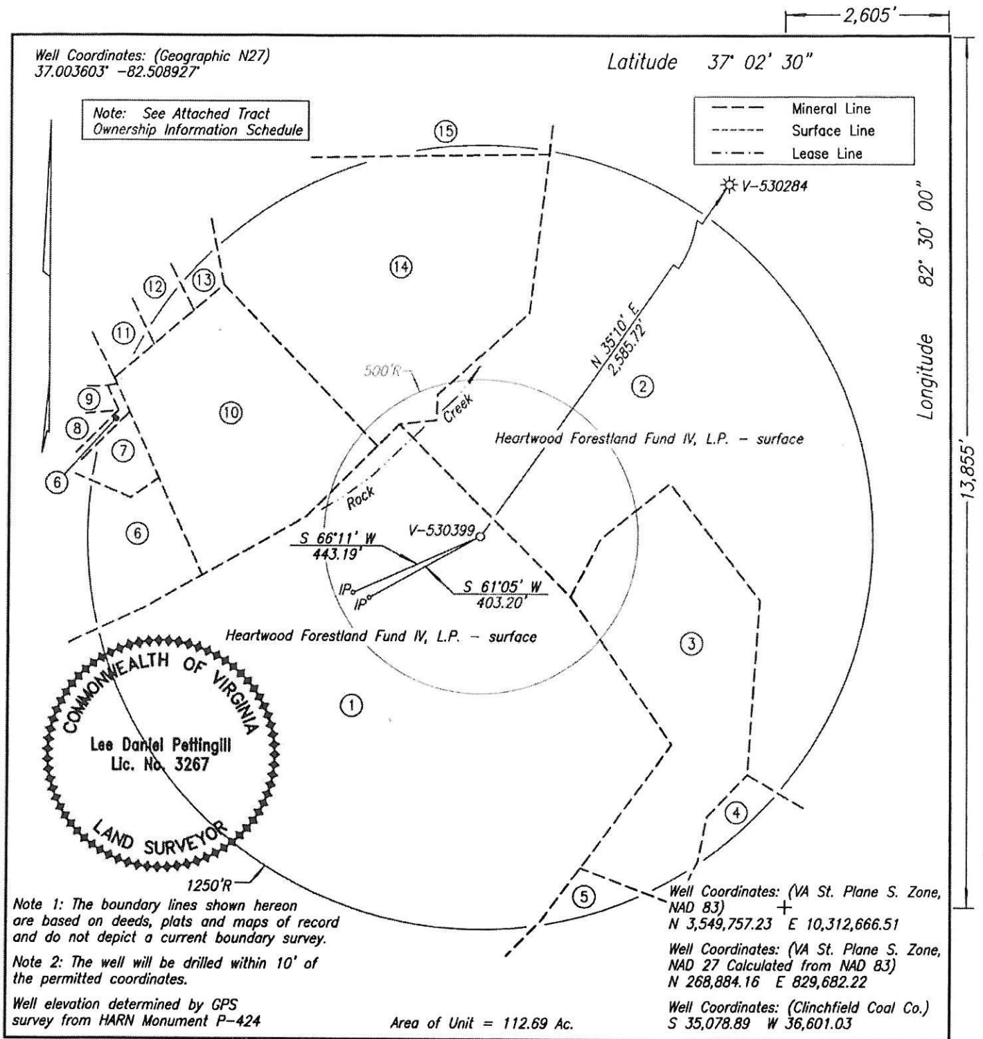
WELL LOCATION PLAT NORA GRID BW-14
